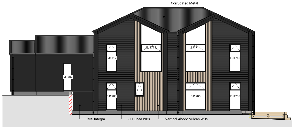
2 Lot 17 - North Elevation
