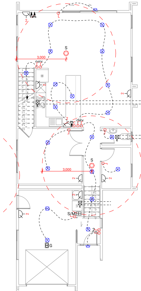
Lower Electrical Plan
