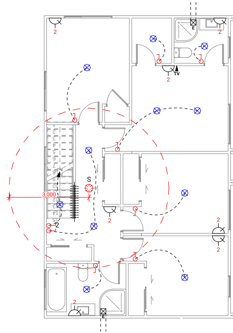
Upper Electrical Plan
