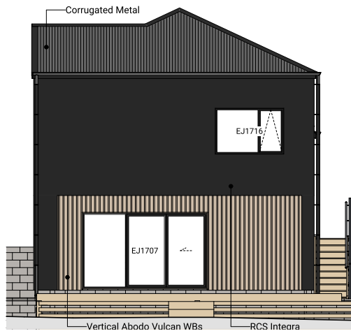
3 Lot 17 - West Elevation
