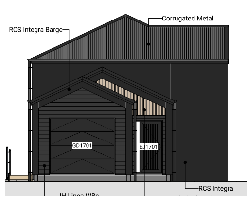
1 Lot 17 - East Elevation
